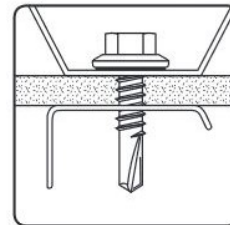
Purlin Screw
